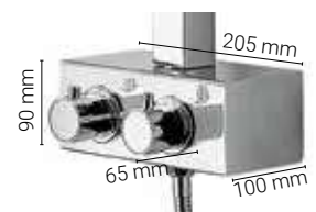
Termostatico in acciaio inox. Interasse 150 mm. Stainless steel thermostatic mixer. Interaxis distance 150 mm.
