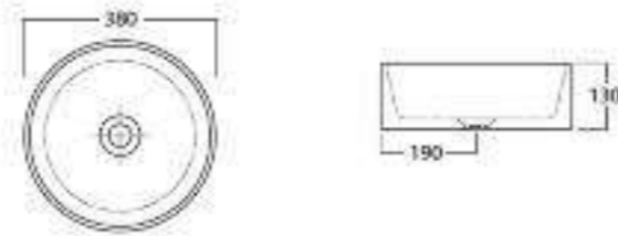
Art. 3154 Vanity Star Round diam cm.38x h.13 Round counter top washbasin cm.38x13h
