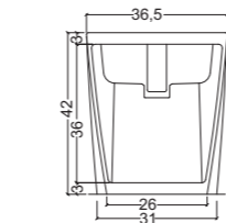
Art. 0552 Bidet Broadway Broadway bidet
