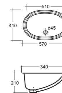
Art. 2703 Lavabo incasso sottopiano Praga cm.57x41 Praga fitted under counter top washbasin cm.57x41
