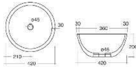
Art. 3111 Lavabo appoggio Harlem cm.42 Harlem counter top basin cm.42
