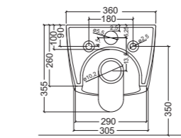
Art. 0652 Vaso Broadway sospeso Broadway wall hung wc bowl
