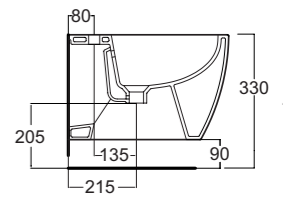
Art. 0750 Bidet sospeso Soho Soho wall hung bidet bowl
