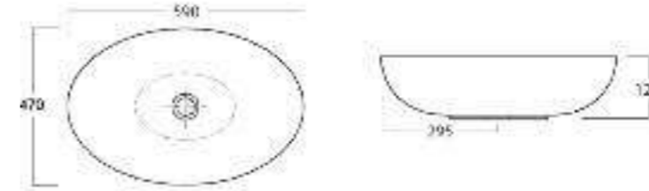
Art. 3142 Vanity Open 59x47 cm.appoggio Vanity Open counter top basin 59x47 cm.
