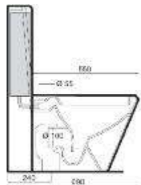
Art. 0352 Cassetta monoblocco a colonna per vaso a terra. Column cistern monoblock for wc back to wall.
