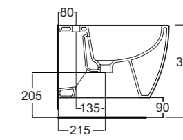
Art. 0750 Bidet sospeso Soho Soho wall hung bidet bowl
