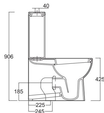
Art. 0250 Vaso monoblocco Soho Soho wc monobloc Art. 0350 Cassetta monoblocco Soho Soho cistern for wc monobloc
