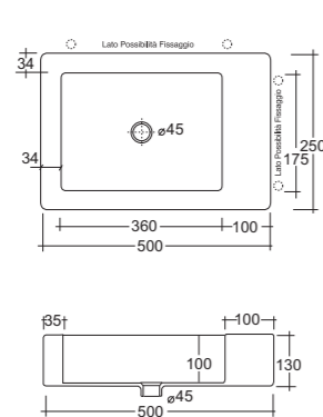
Art. 3103 Lavabo appoggio Quadro cm.50x25 Square counter top basin cm.50x25
