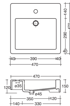
Art. 3106 Lavabo Quadro semincasso cm.47x47 Square semi-mounted washbasin cm.47x47
